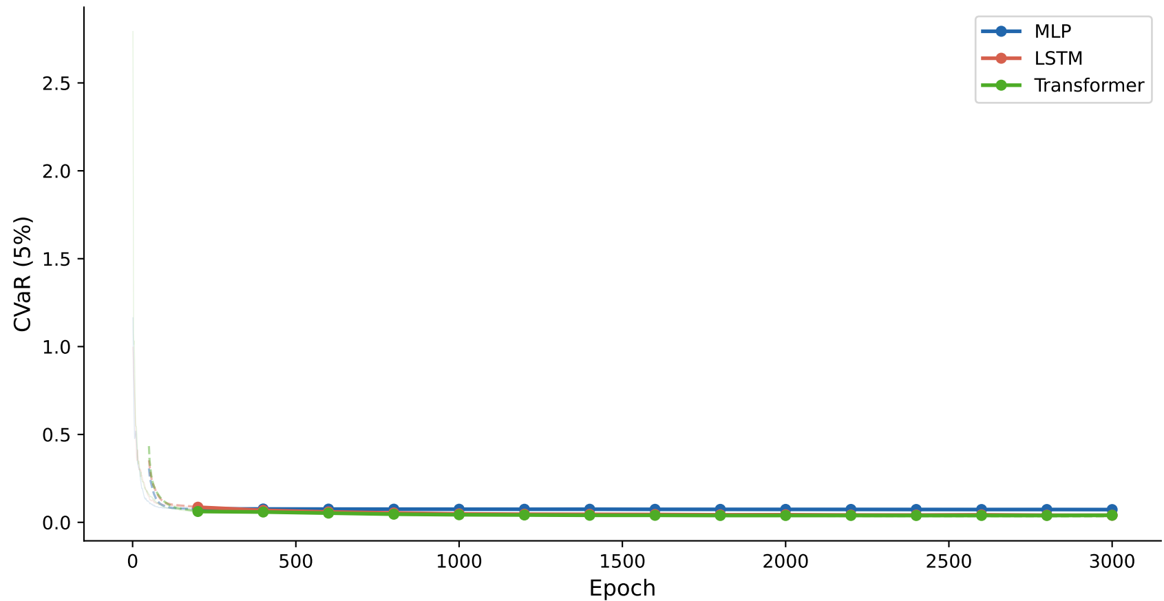
CVaR convergence -- REDUCED features (dashed = train MA-50; solid = eval every 200 epochs)
