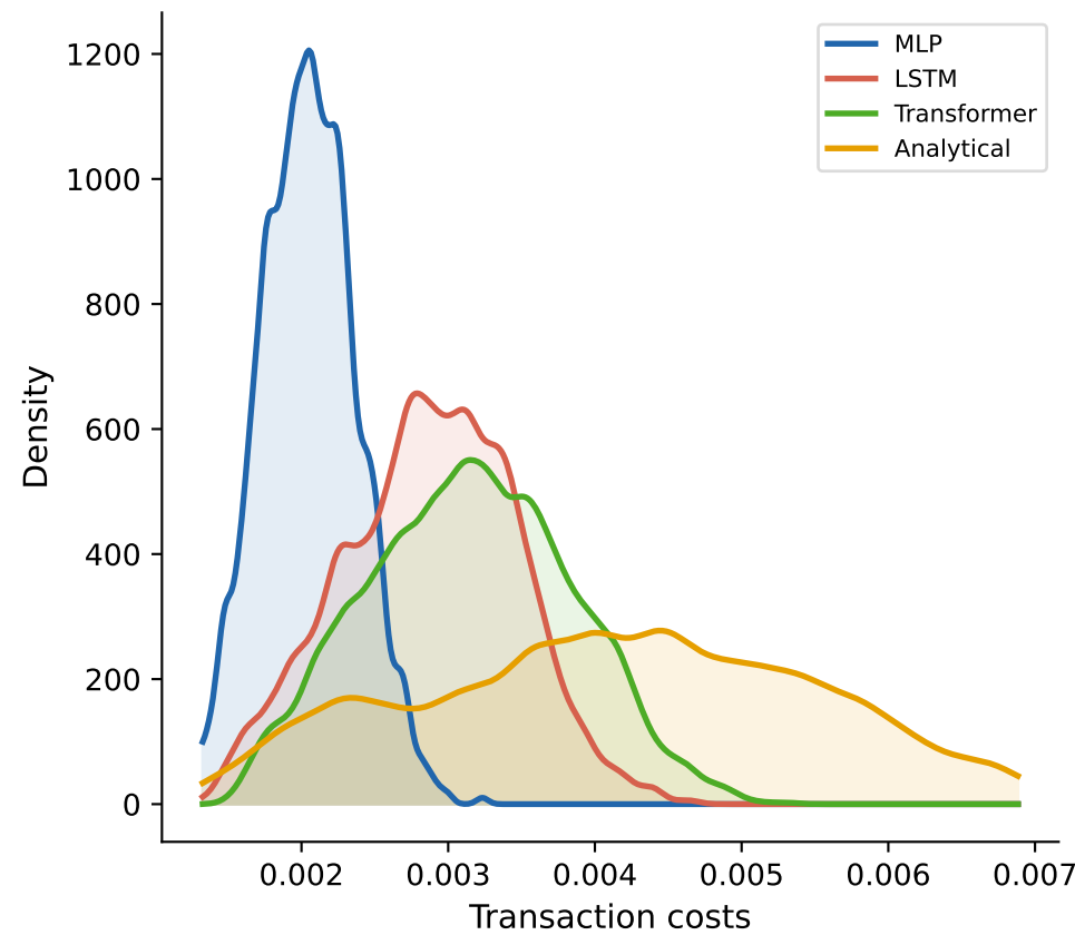
Transaction cost distributions REDUCED features
