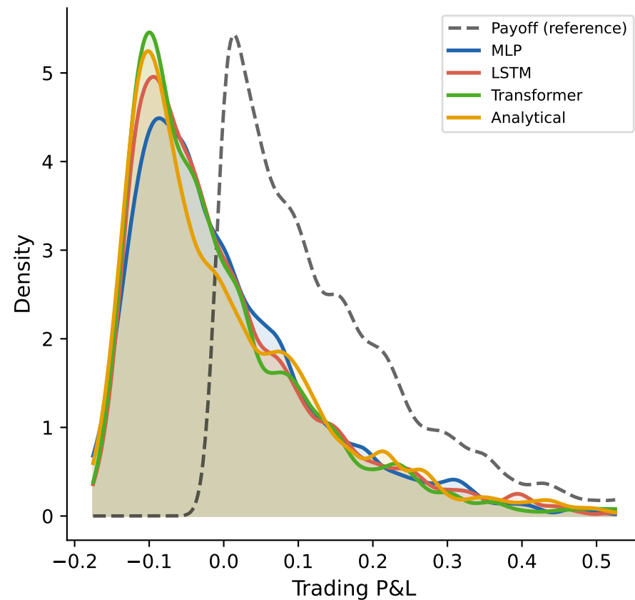
Trading P&L vs Payoff (dashed) REDUCED features
