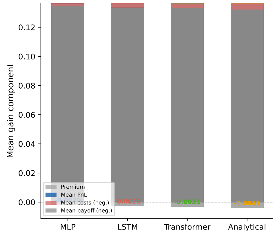
Mean gain attribution REDUCED features
