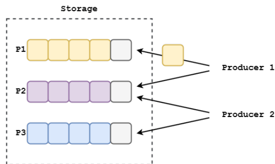
Figura 4.6: Partition
