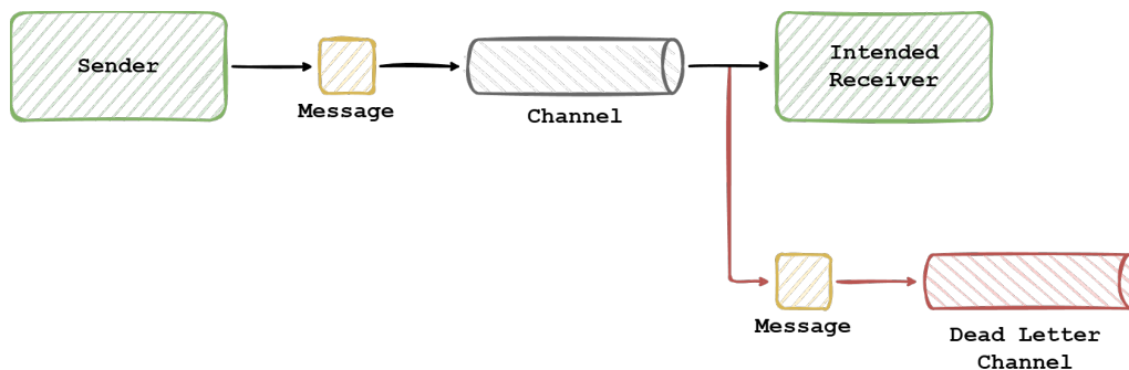
Figura 4.2: Dead Letter Channel
