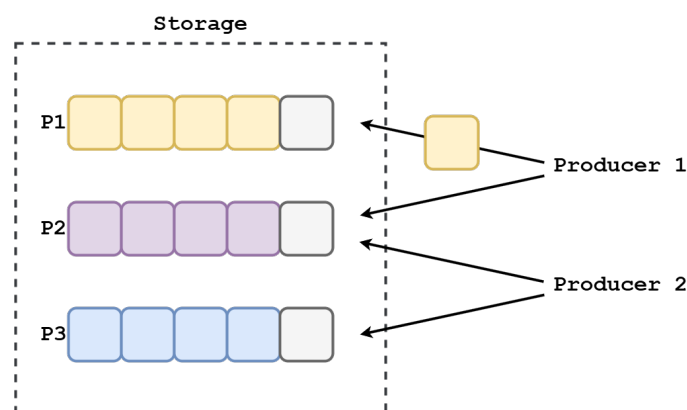
Figura 4.6: Partition
