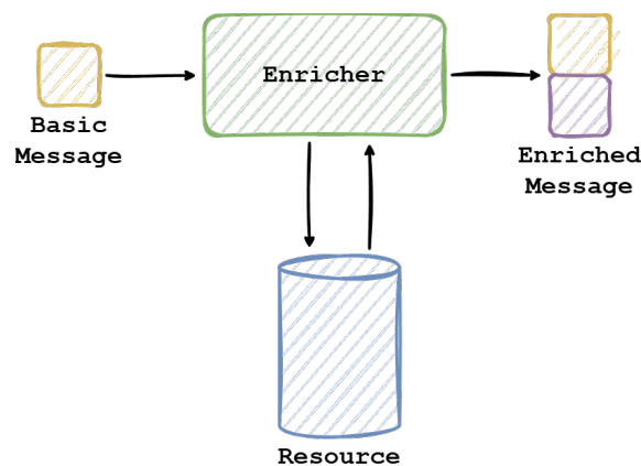
Figura 4.1: Content Enricher
