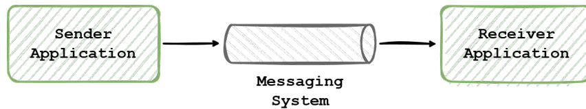
Figura 4.3: Message Channel
