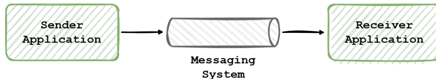
Figura 4.3: Message Channel
