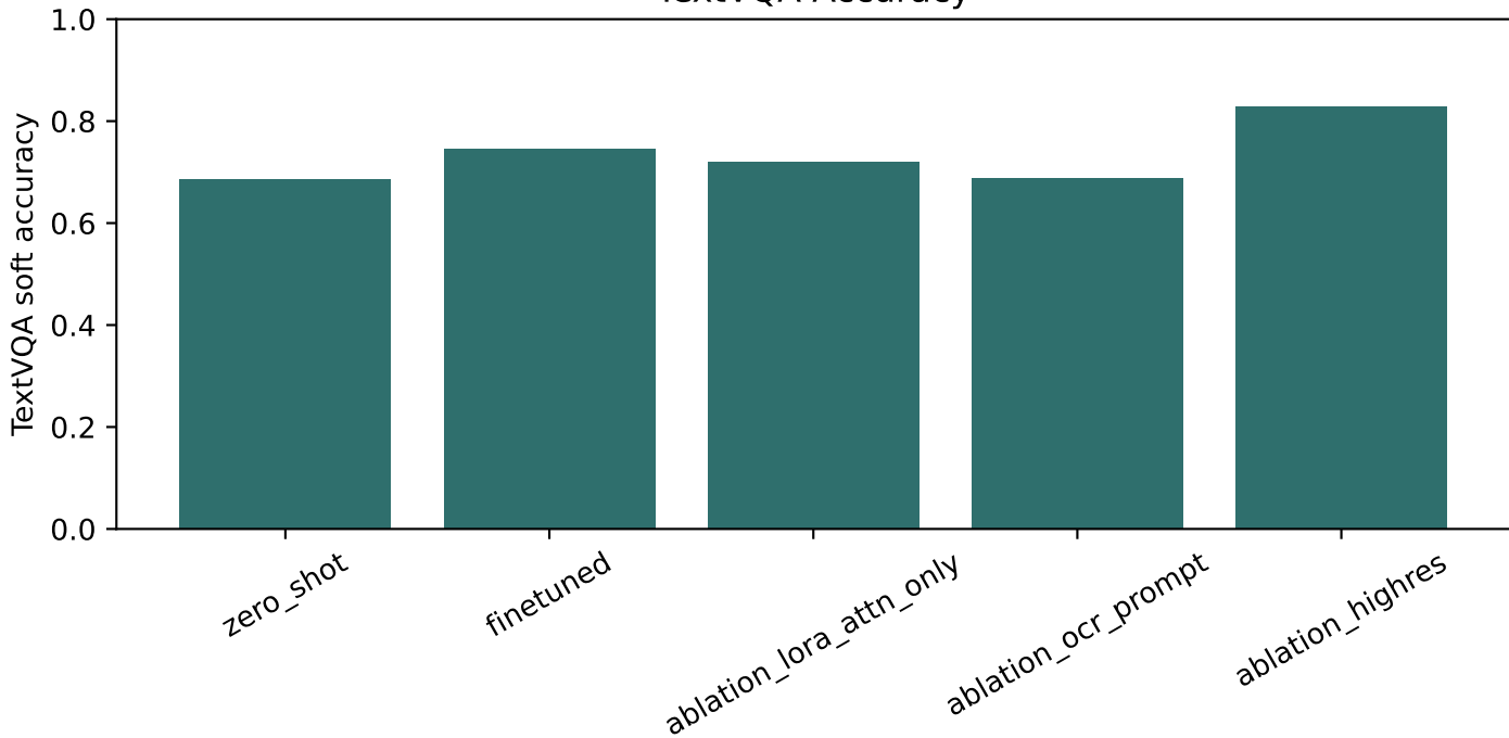
TextVQA Accuracy
