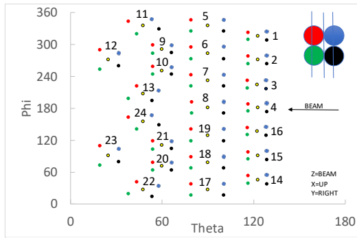
CLARION-A (Master)
