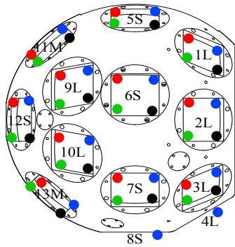
CLARION-A (Master)
