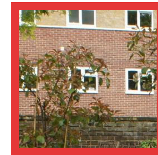
Ground Truth
