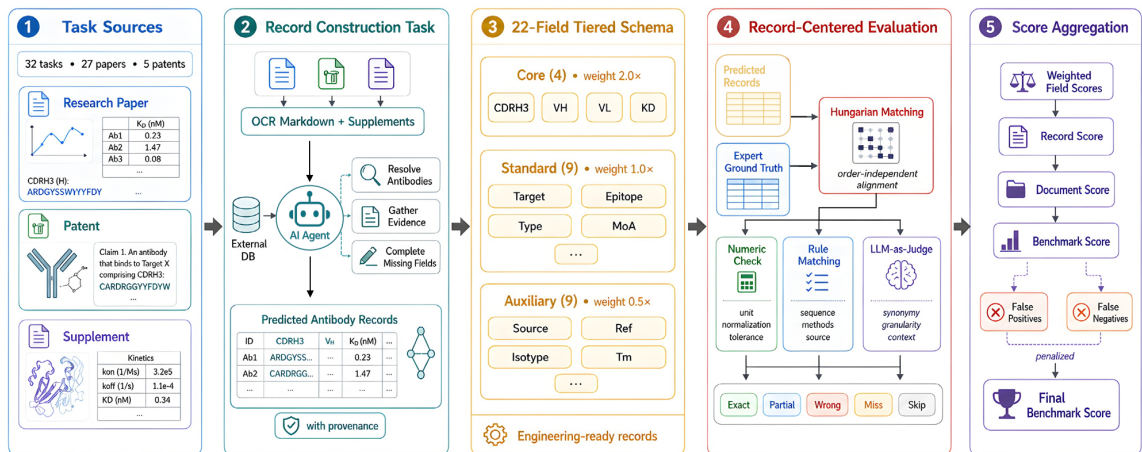
Figure 2: ABDBENCH benchmark workflow . Papers, patents, and supplementary materials are processed by the extraction agent to produce structured antibody records under the 22-field tiered schema. Predicted records are then compared with expert records through order-independent record alignment, deterministic field checks, LLM adjudication, weighted aggregation, and false-positive and false-negative penalties to obtain final scores.
