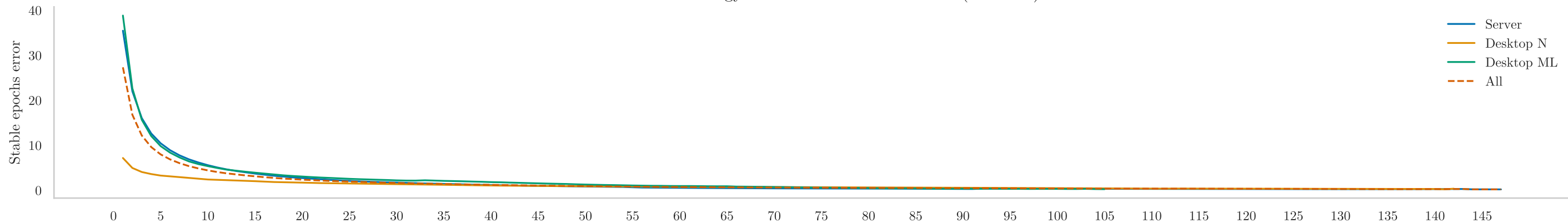
RMSE of the energy estimation vs. window size (STEP-P)
