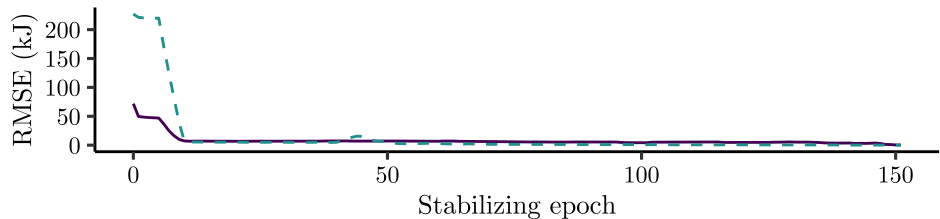
RMSE of energy estimation vs. stabilizing epoch
