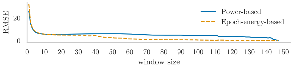
RMSE of the energy estimation vs. window size
