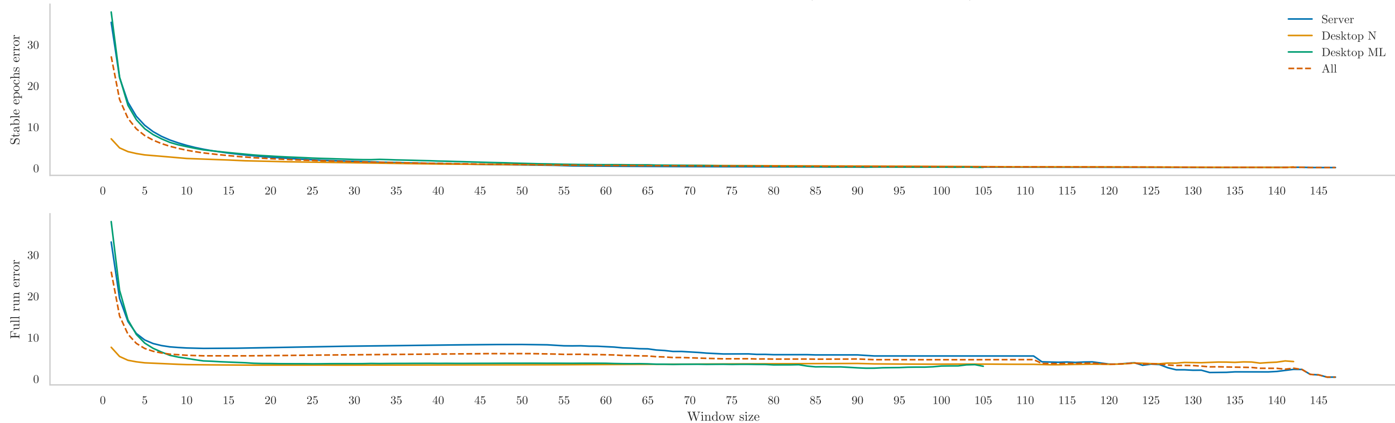
RMSE of the energy estimation vs. window size (power-based estimator)
