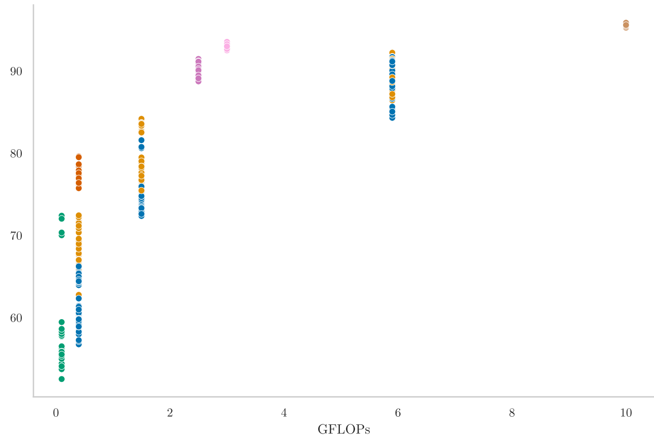
Desktop ML
