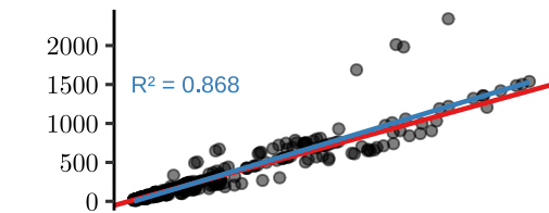
Green Algorithms
