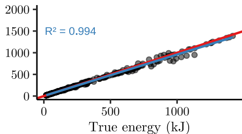
Offline Power-based
