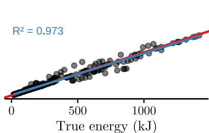
Offline Energy-based
