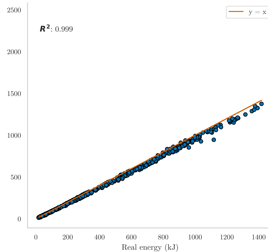
Online epoch-energy-based estimator
