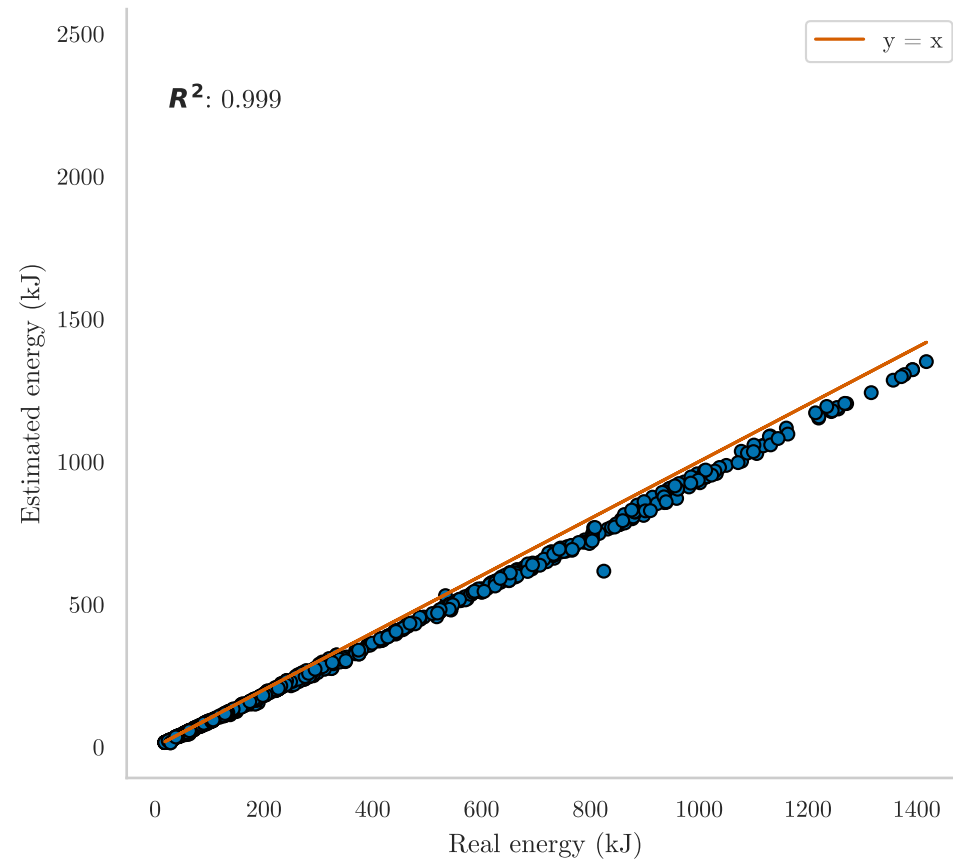
Online power-based estimator
