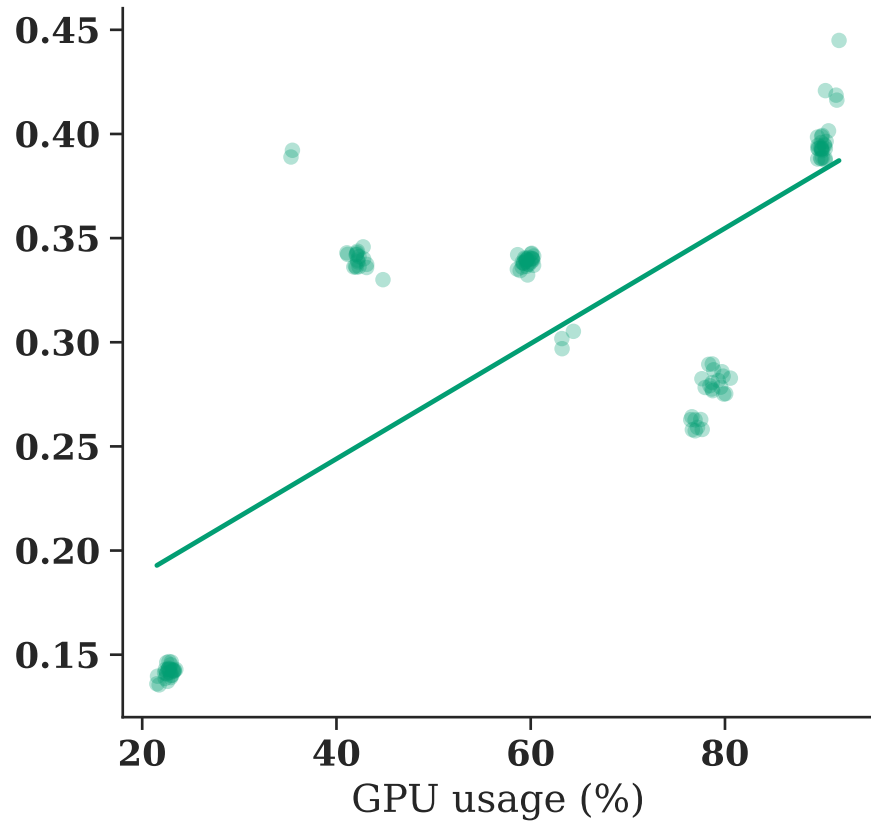
Server
