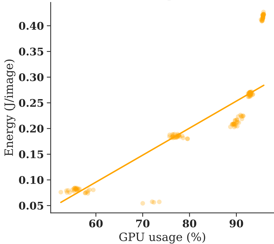
Desktop ML
