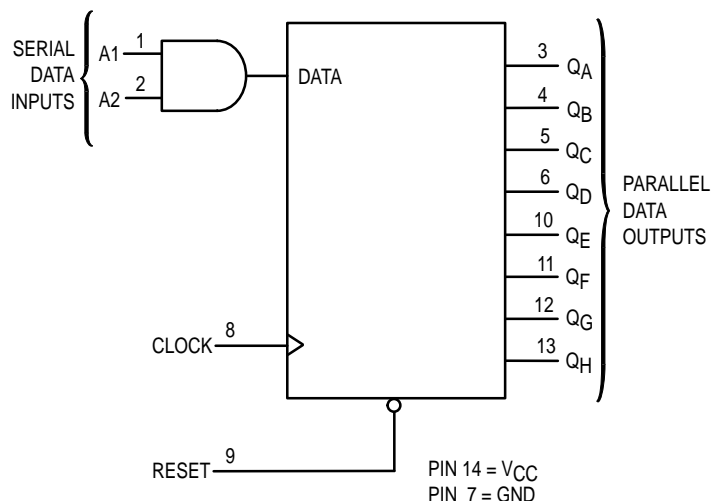
LOGIC DIAGRAM
