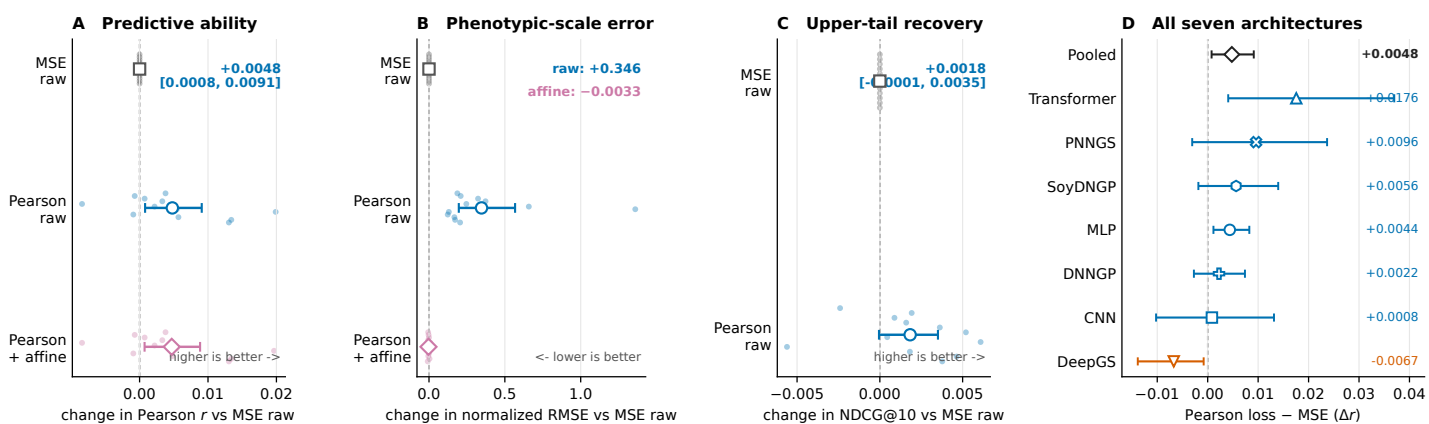
Figure 4 The central empirical comparison. Panels A–B show that raw Pearson predictions gain 0.0048 in correlation but increase normalized RMSE by 0.346 relative to raw MSE; affine calibration retains the correlation gain (+0.0047) and removes the scale penalty (−0.0033). Panel C shows that raw NDCG@10 changes by only +0.0018. Panel D reports estimates and 95% panel-cluster bootstrap intervals for the pooled result and all seven architectures. Small points in A–C are contrasts for the 12 panels.
