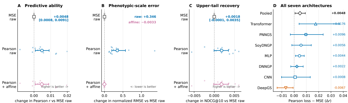
Figure 4 The central empirical comparison. Panels A–C show that raw Pearson predictions gain 0.0048 in correlation but increase normalized RMSE by 0.346 relative to raw MSE; affine calibration retains the correlation gain (+0.0047) and removes the scale penalty (−0.0033), while raw NDCG@10 changes by only +0.0018. Panel D reports estimates and 95% panel-cluster bootstrap intervals for the pooled result and all seven architectures. Small points in A–C are contrasts for the 12 panels.
