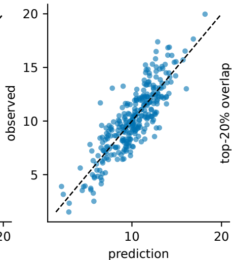
affine-calibrated r=0.85 , RMSE=1.58
