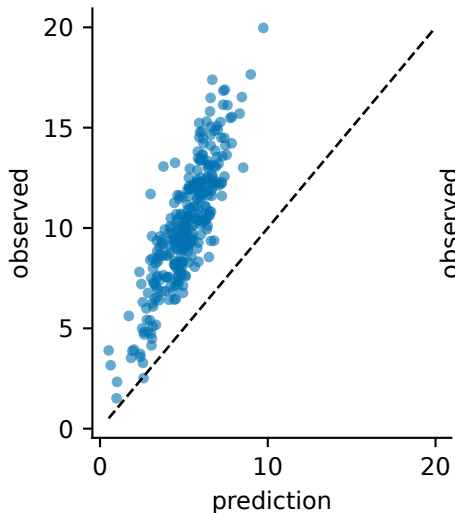
raw prediction r=0.85 , RMSE=5.38
