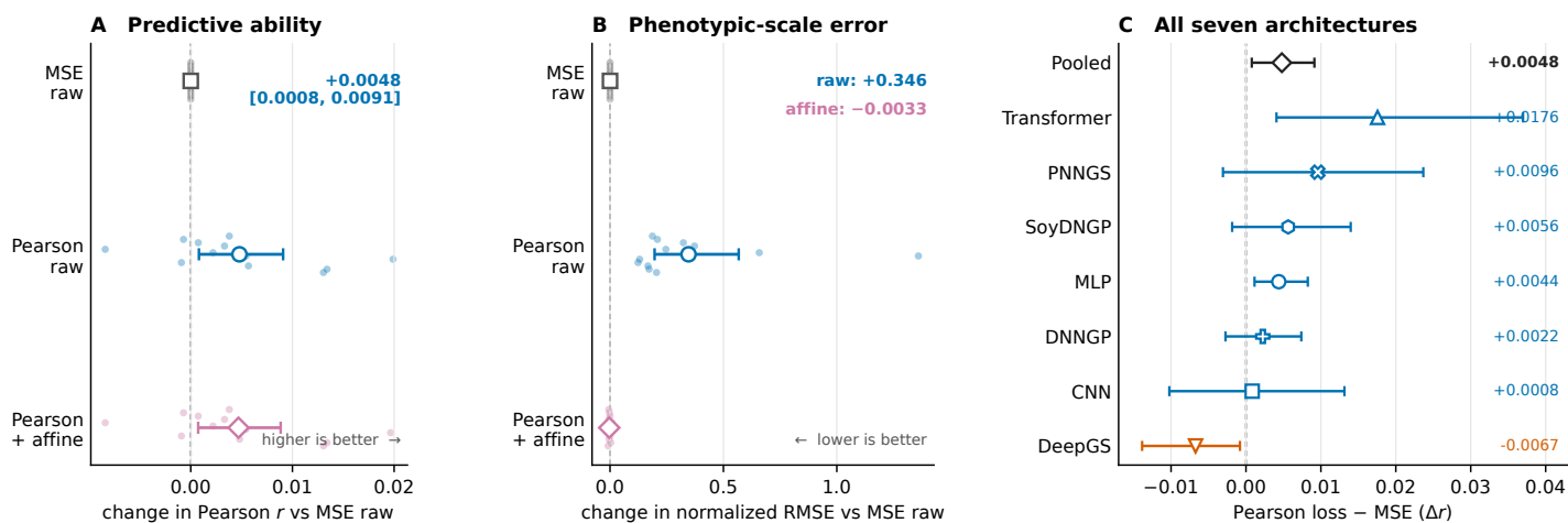
Figure 4 The central empirical comparison. Panels A–B show that raw Pearson predictions gain 0.0048 in correlation but increase normalized RMSE by 0.346 relative to raw MSE; affine calibration retains the correlation gain (+0.0047) and removes the scale penalty (−0.0033). Panel C reports estimates and 95% panel-cluster bootstrap intervals for the pooled result and all seven architectures. Small points in A–B are contrasts for the 12 panels.
