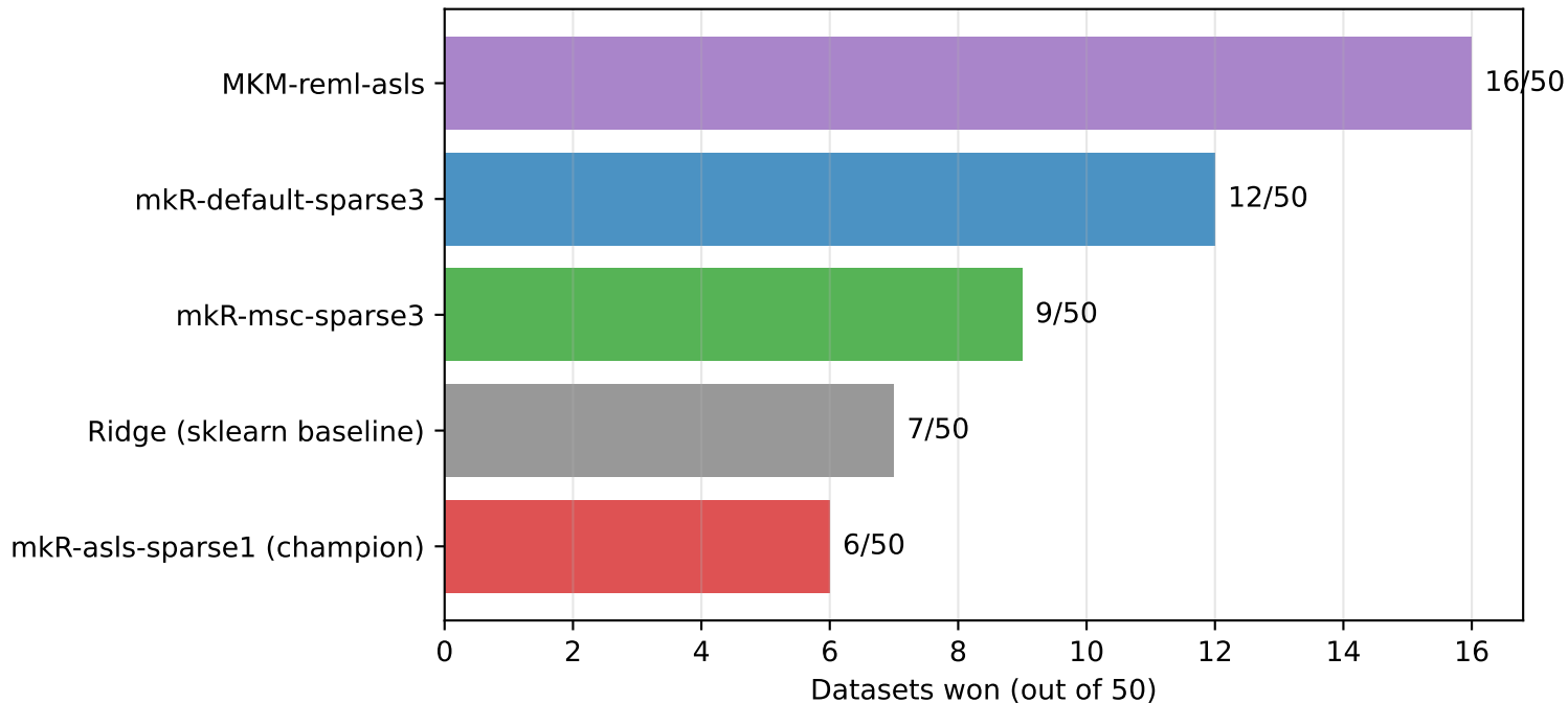
Iter 8: oracle variant frequency (best variant per dataset)
