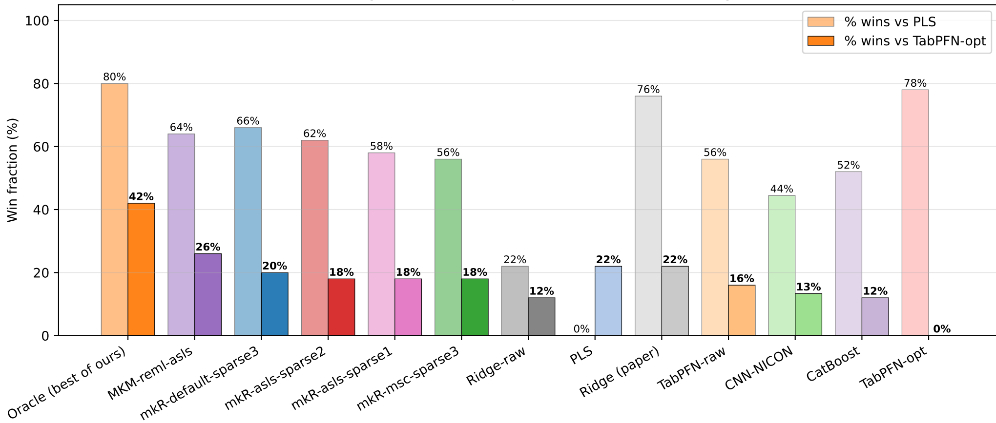
Win rate vs PLS (light) and TabPFN-opt (dark) — across ~50 Stage A datasets
