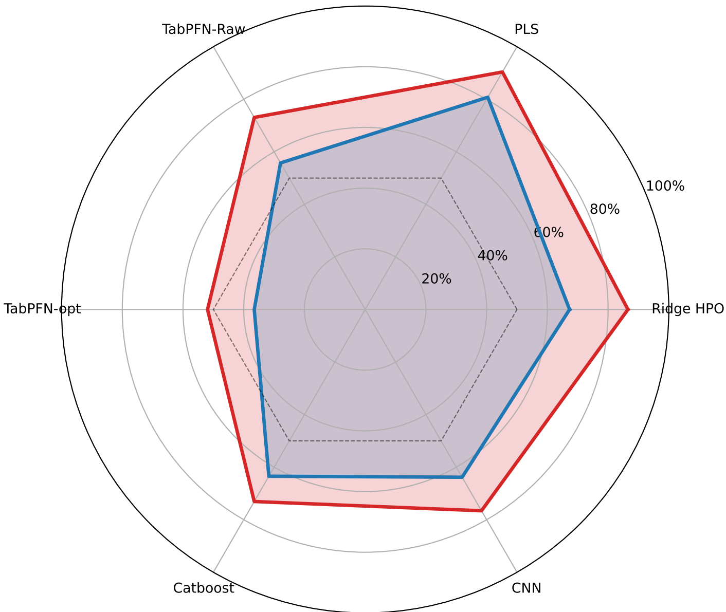
Win-rate of AOM-Ridge variants vs. TabPFN-paper baselines (52 datasets; 50% dashed line = tie)
