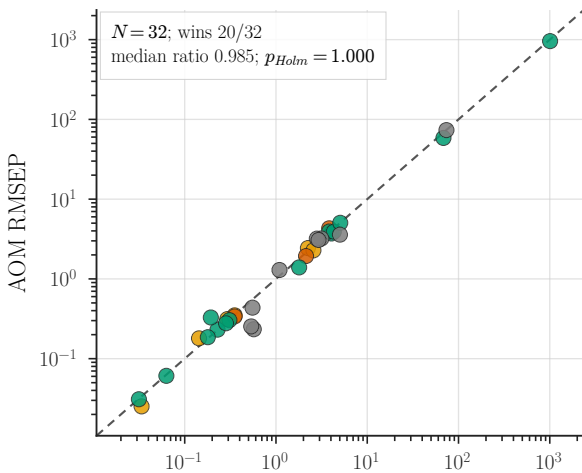
AOM-Ridge best vs Ridge-default
