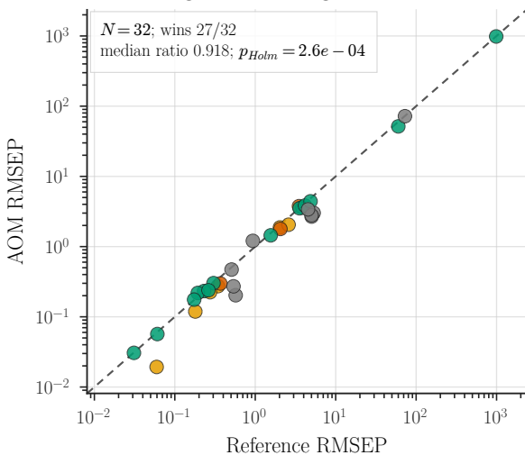
AOM-Ridge best vs Ridge-default
