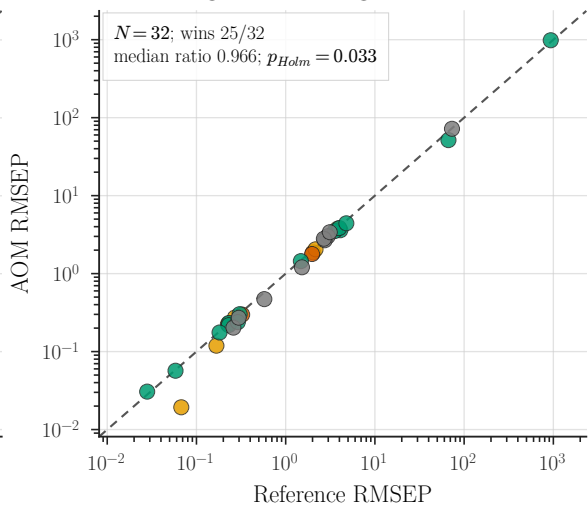
AOM-Ridge best vs Ridge-HPO
