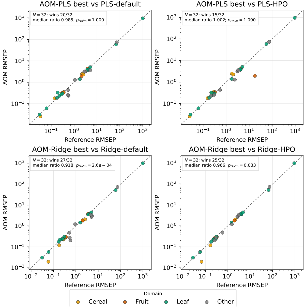
Figure 5: Prediction-quality scatter plots for the selected AOM-PLS and AOM-Ridge variants against default and HPO references. Axes are log RMSEP; points below the diagonal favour AOM.
