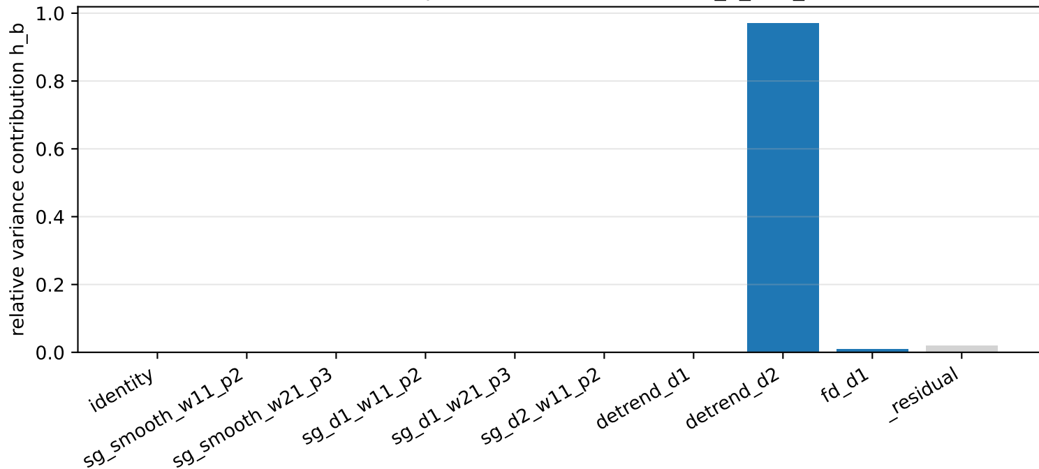
MKM/BLUP variance decomposition — ALPINE/ALPINE_P_291_KS (branch=asls)
