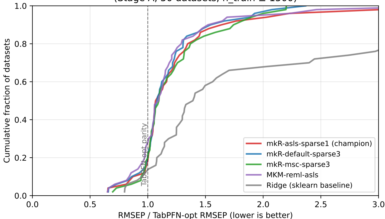
Iter 8: cumulative distribution of relative RMSEP vs TabPFN-opt (Stage A, 50 datasets, n_{\text{train}} \leq 1500 )
