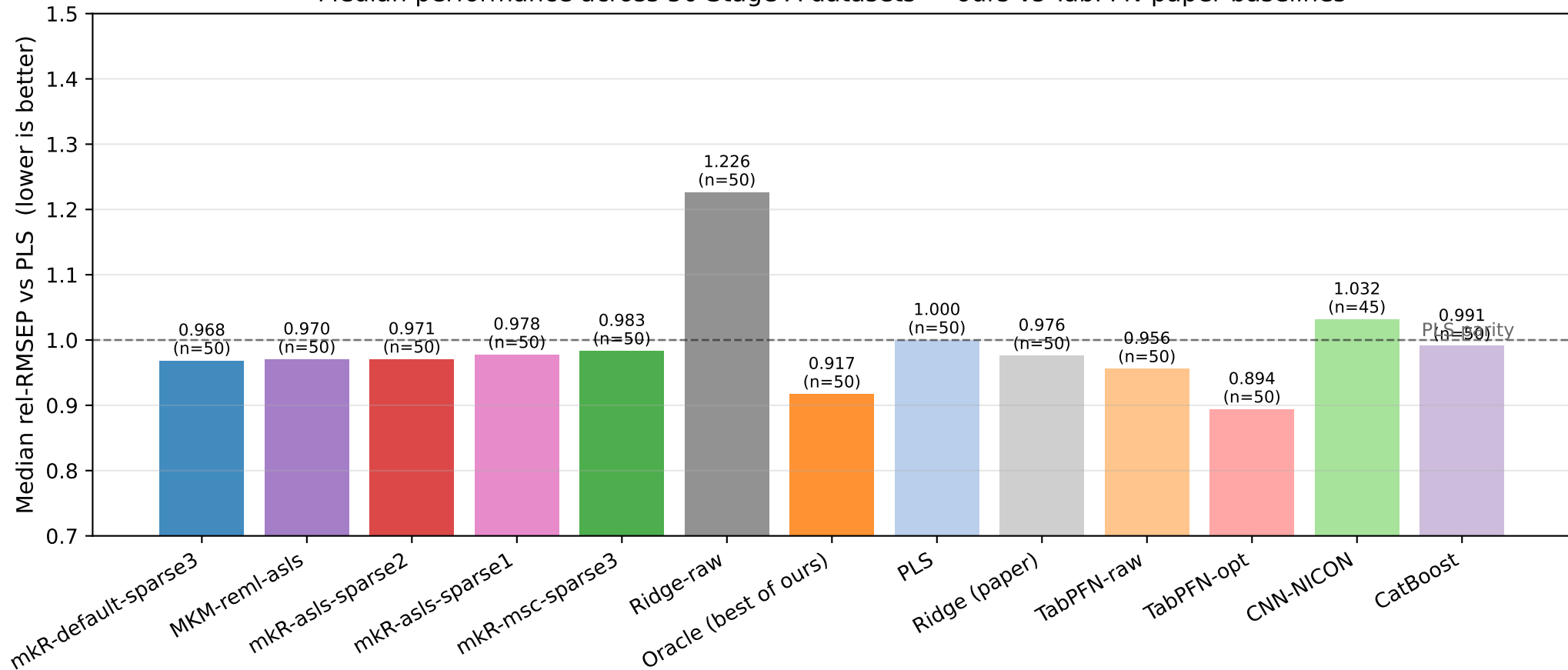
Median performance across 50 Stage A datasets — ours vs TabPFN-paper baselines
