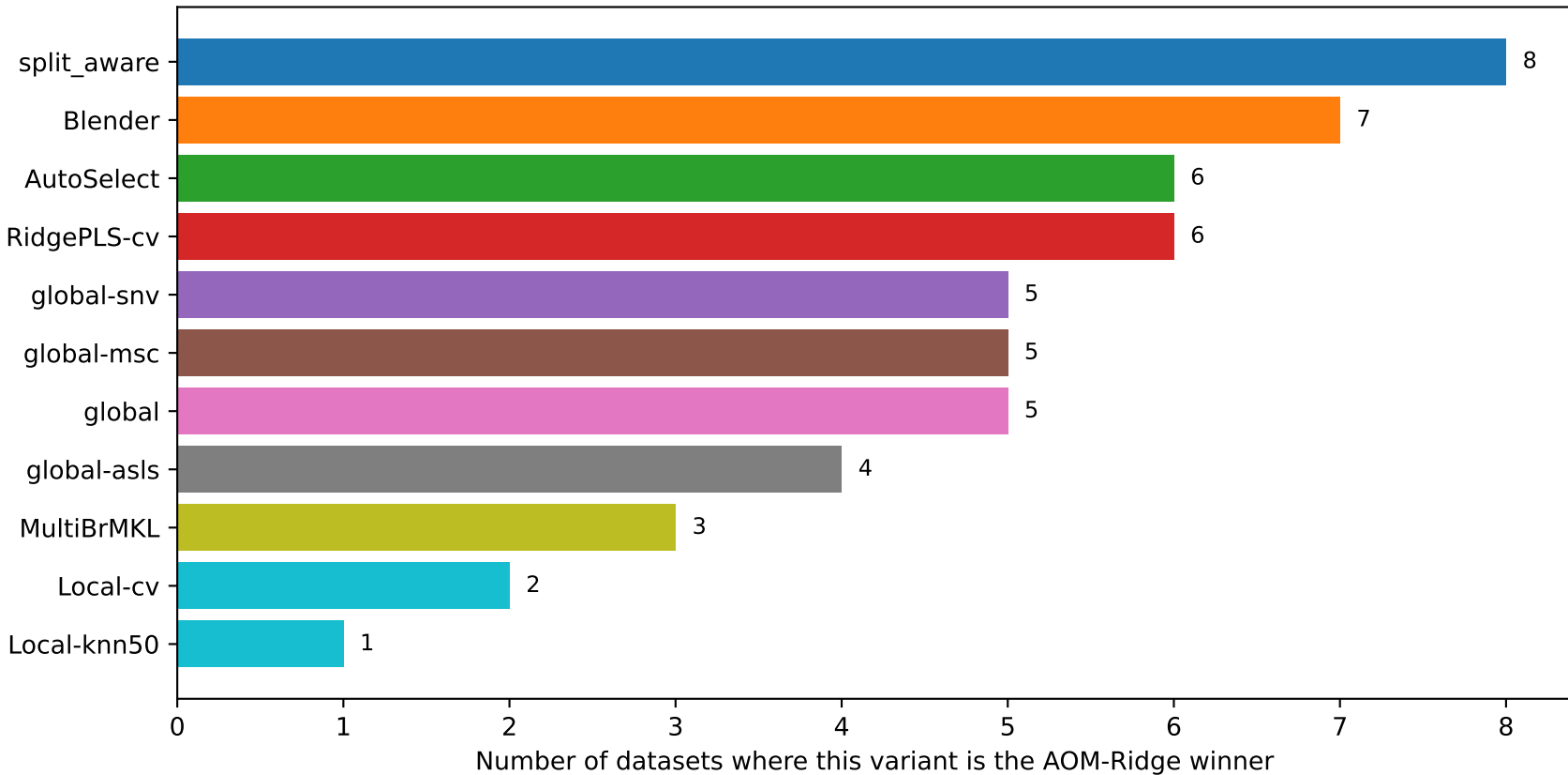
Per-dataset winner among AOM-Ridge top variants (52 datasets, top variants only)
