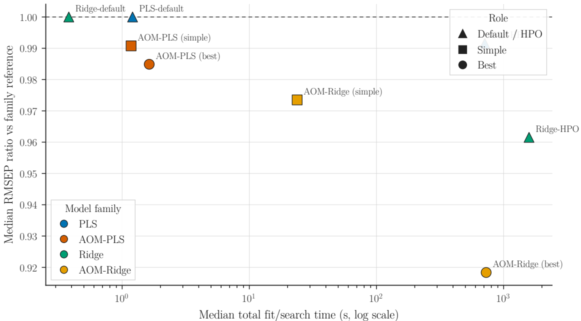
Accuracy / time Pareto
