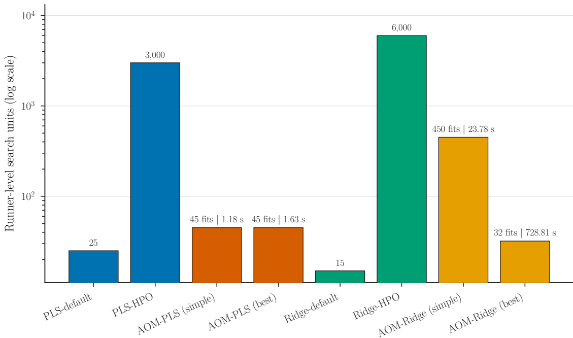
Search-budget scale
