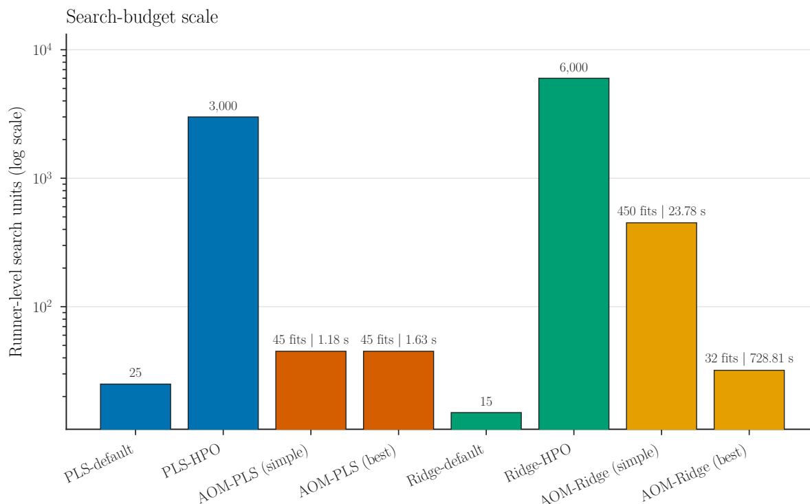
Figure 7: Search-budget scale for the eight paper variants: PLS-default, PLS-HPO, AOM-PLS (simple), AOM-PLS (best), Ridge-default, Ridge-HPO, AOM-Ridge (simple) and AOM-Ridge (best). Counts are runner-level search units: logged trials for PLS/Ridge defaults and HPO, compact-bank CV fits for AOM-PLS, operator-alpha cells for AOM-Ridge (simple), and top-level outer-selector fits plus refits for AOM-Ridge (best).
