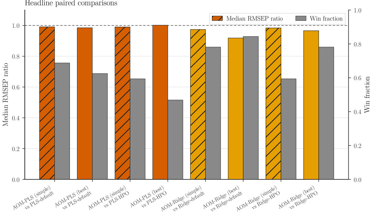
Figure 4: Eight paired regression comparisons for the plain compact-bank AOM baselines and the selected AOM-PLS and AOM-Ridge variants against their PLS-default, PLS-HPO, Ridge-default and Ridge-HPO references.
