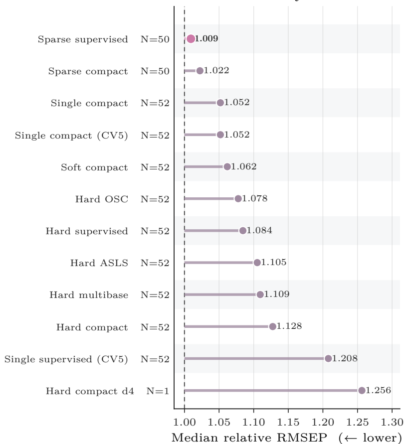
Predictive accuracy
