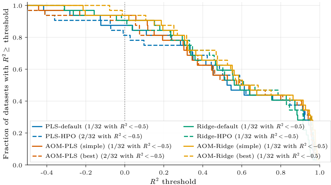
R^2 coverage curve ( N=32 datasets, R^2 clipped at -0.5 )
