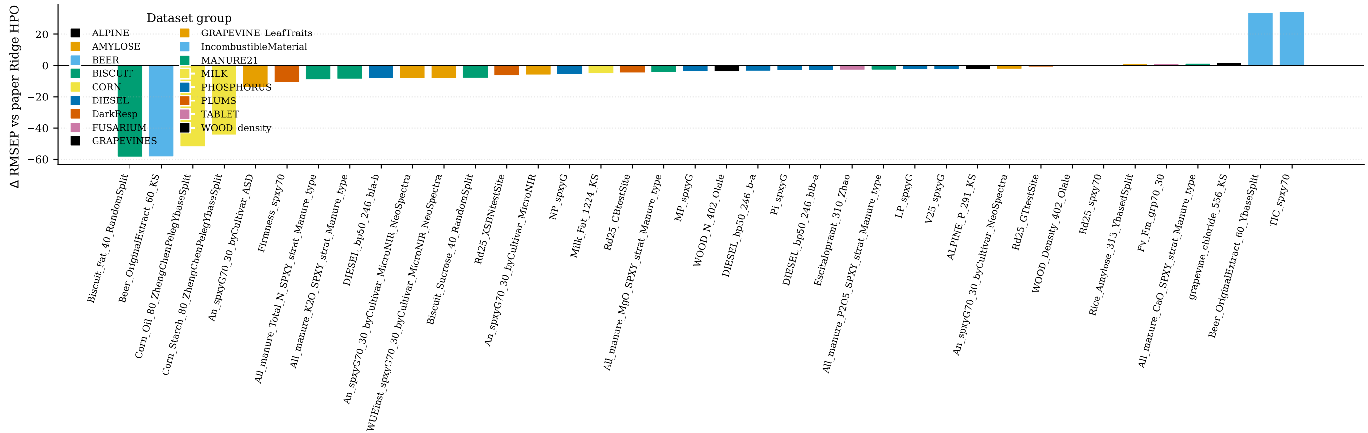
AOM-Ridge (best variant) per-dataset delta vs paper Ridge HPO [31 wins / 7 losses / 38 datasets]
