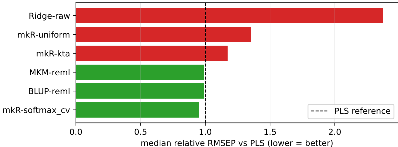
Per-variant median performance — smoke benchmark
