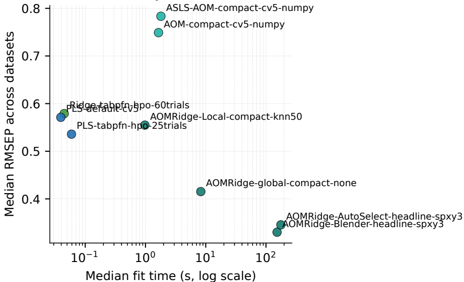
Accuracy vs. fit time
