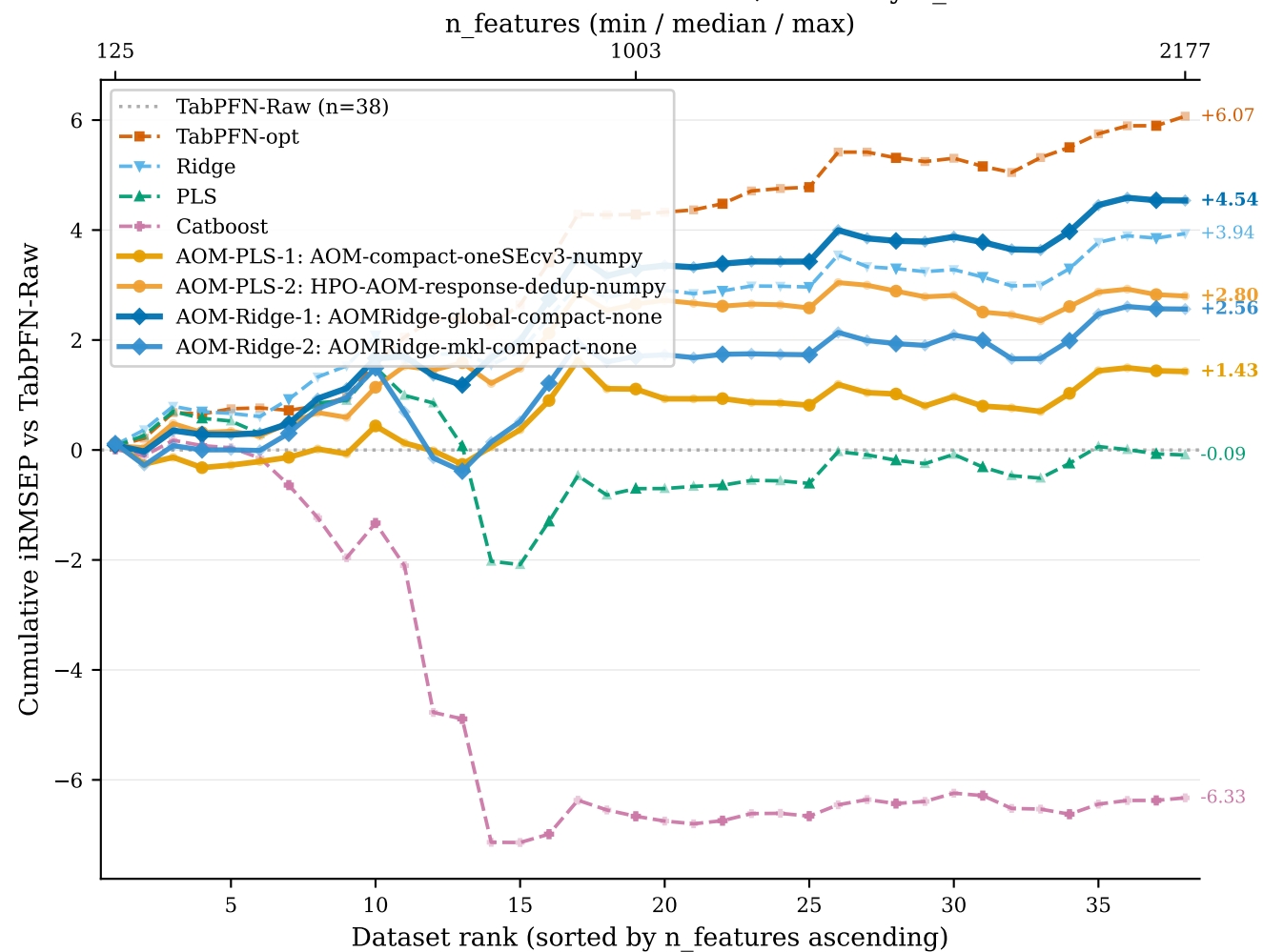
Cumulative iRMSEP vs TabPFN-Raw, sorted by n_features
