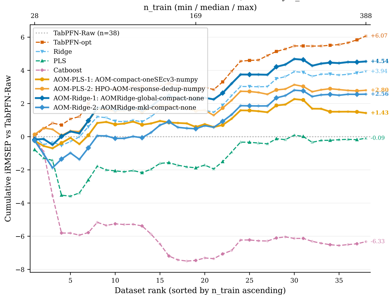
Cumulative iRMSEP vs TabPFN-Raw, sorted by n_train
