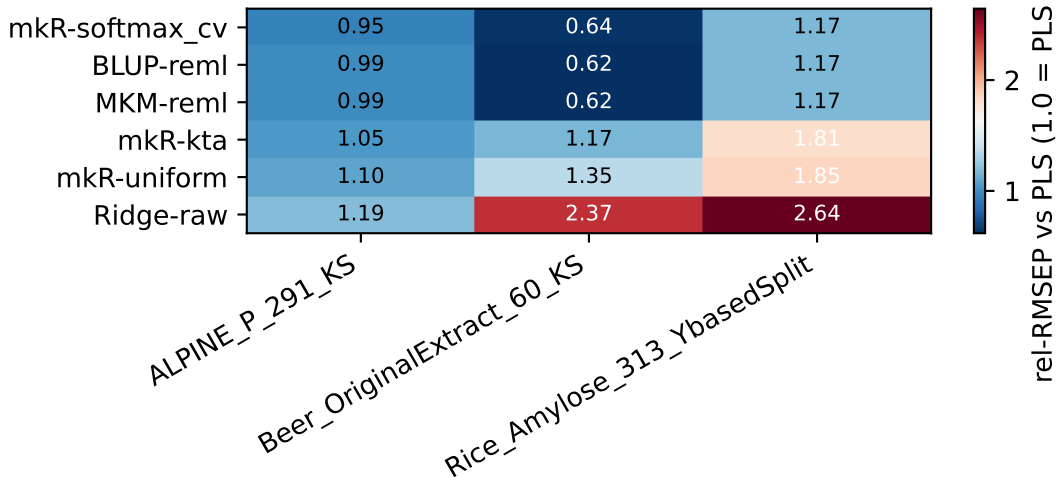
Variant × dataset — relative RMSEP vs PLS
