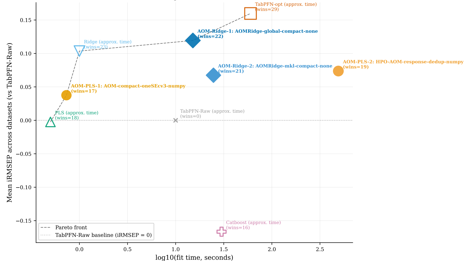
iRMSEP vs training time (mean across datasets)
