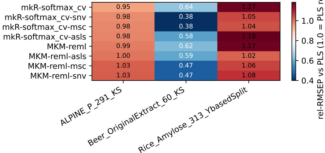
Variant x dataset — relative RMSEP vs PLS
