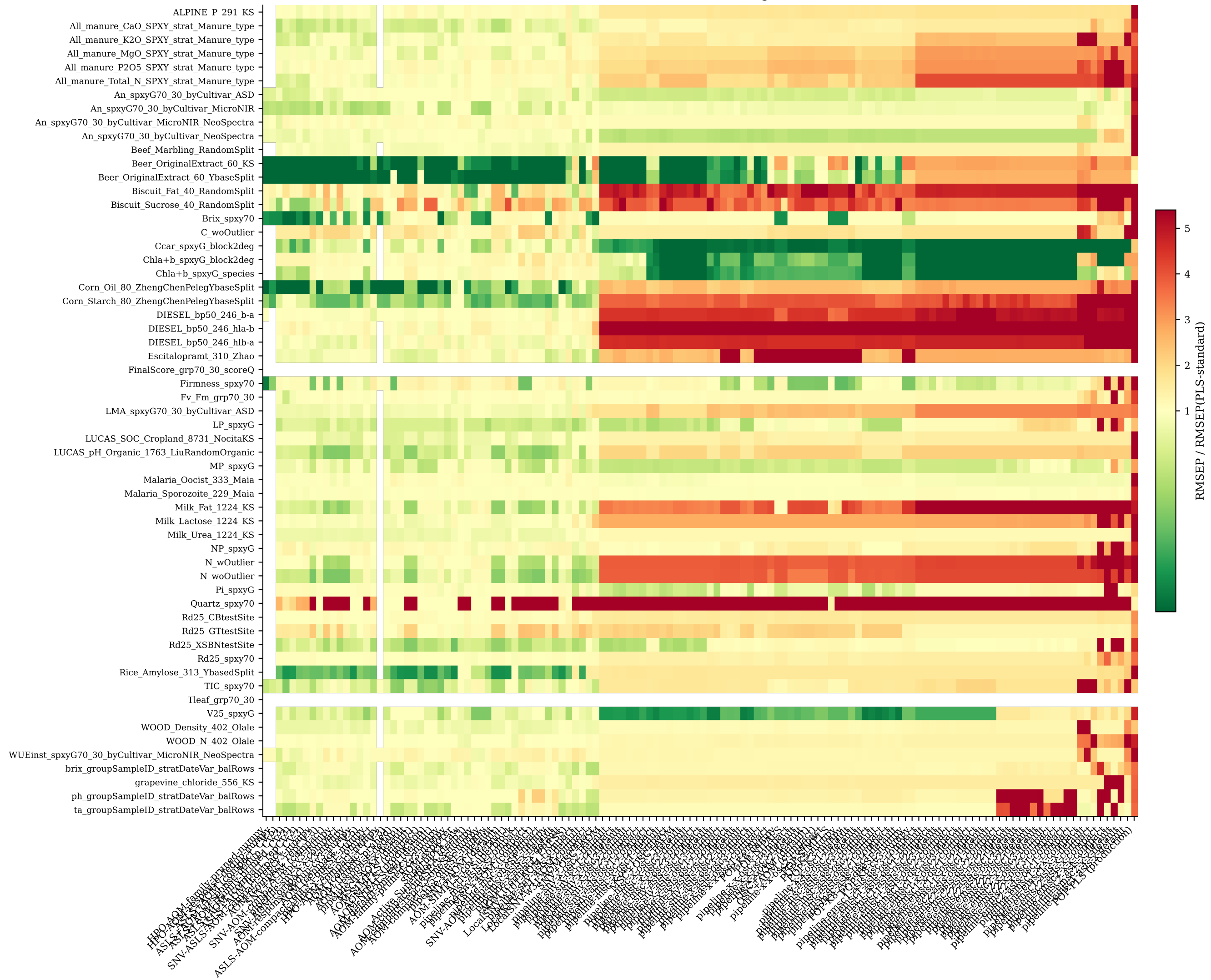
Relative RMSEP / PLS (lower = better, green = beats PLS)
