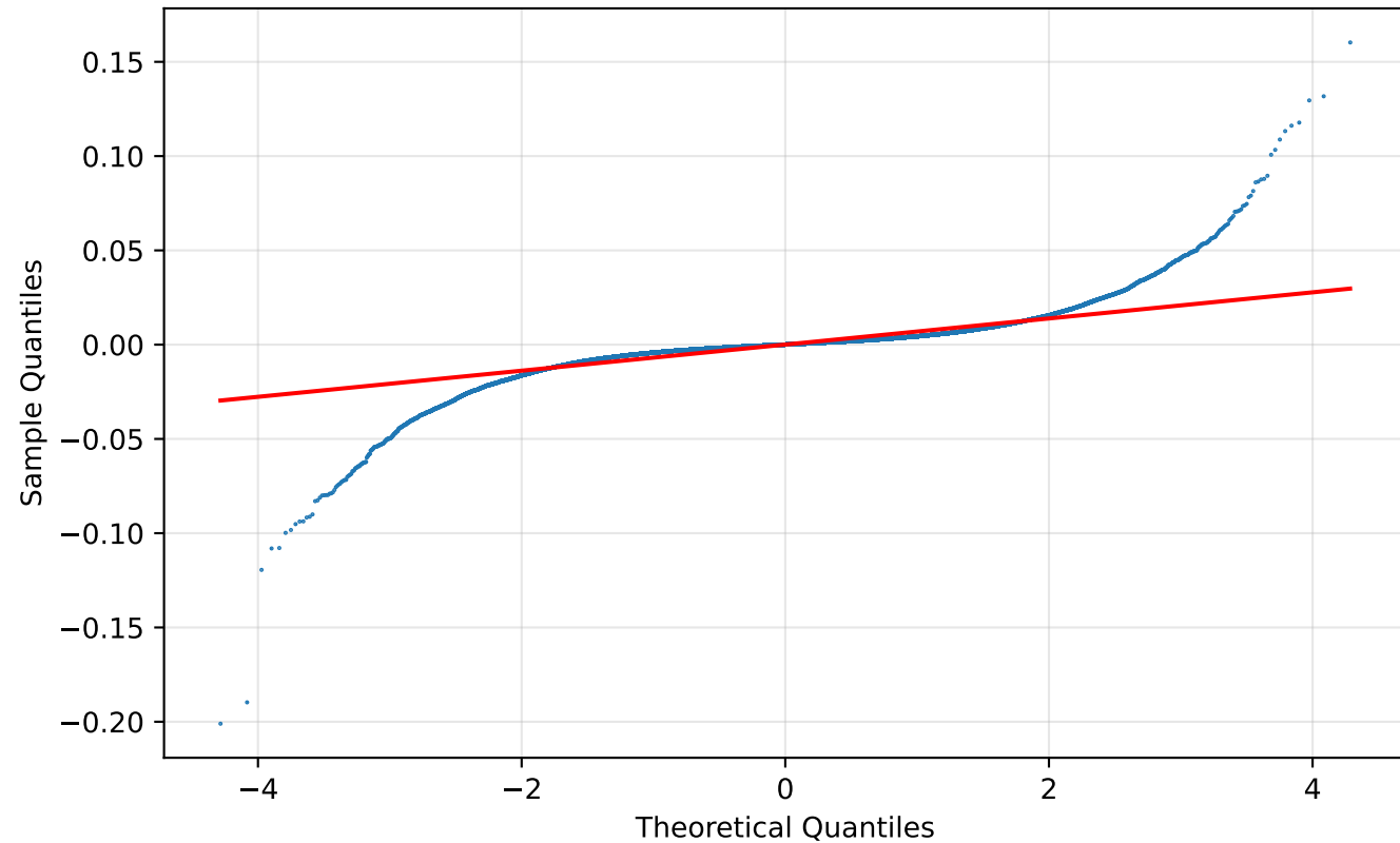
Q-Q Plot vs Normal
