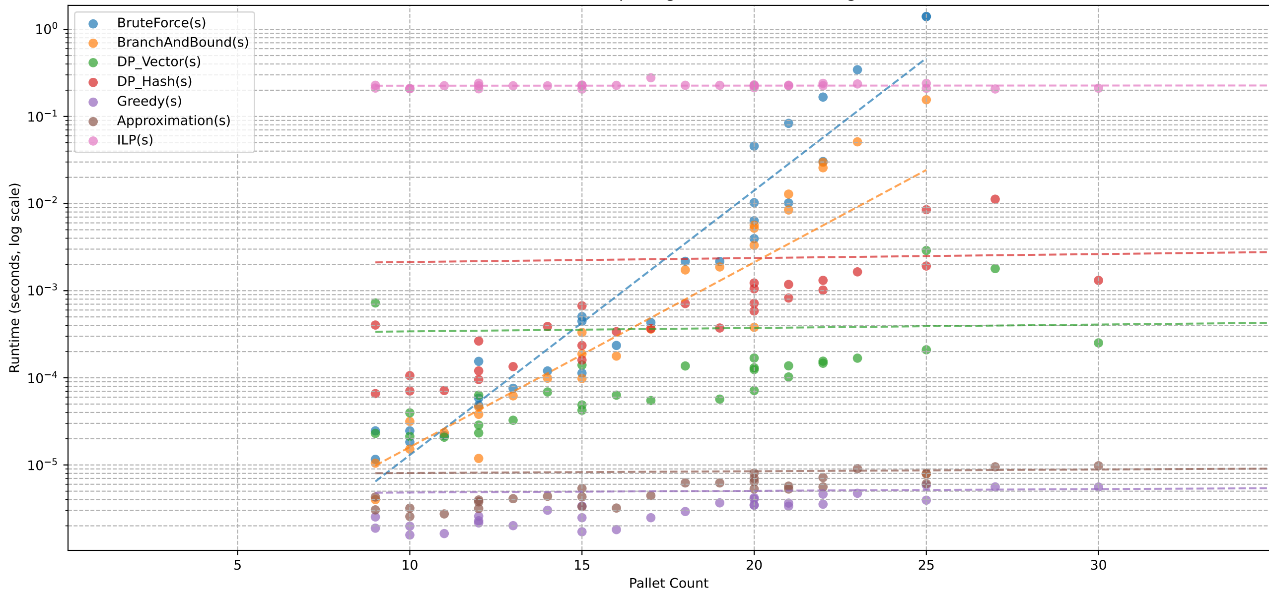
Runtime vs Pallet Count per Algorithm with Linear Regression
