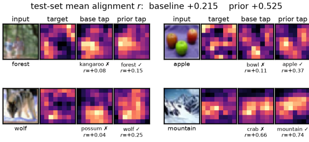
Figure 4: The spectral imprint at the tap, CIFAR-100 at 5%. Each of the four sample blocks shows the input, the fixed moment target, and the tapped-stage energy of the baseline and prior arms. Over the whole test set the alignment between tapped features and the target is +0.215 for the baseline and +0.525 for the prior arm. The four samples are selected cases (prior arm correct, baseline wrong), so they illustrate the alignment difference, not sample it, and only the test-set-wide figure should be read as evidence.
