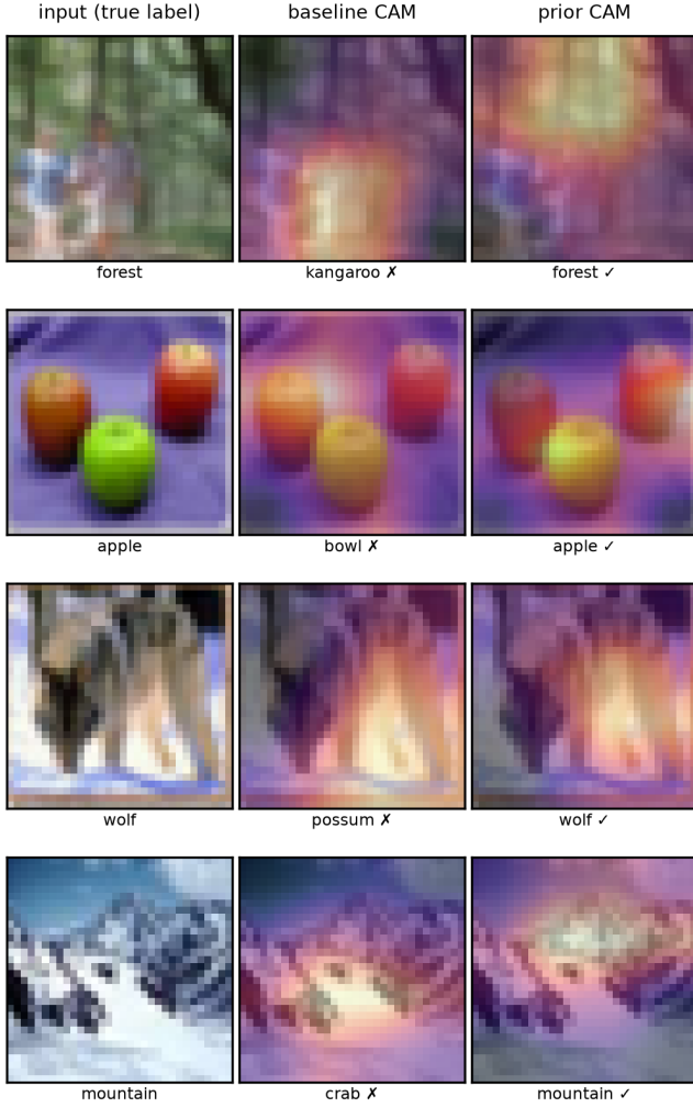
Figure 8: Class-activation maps, CIFAR-100 at 5%, for four selected test images (prior arm correct, baseline wrong). The prior arm’s evidence concentrates on object contours and texture boundaries where the baseline’s is diffuse at this data scale.
