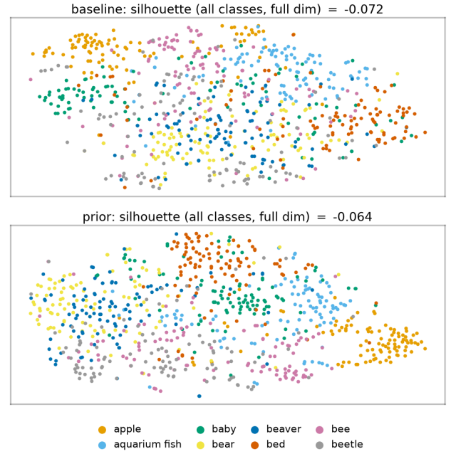
Figure 9: t-SNE of frozen penultimate test features, first eight classes, baseline (top) and prior arm (bottom) at the CIFAR-100 5% cell. The silhouette in each title is computed over all classes in the full feature space, not on the two projected dimensions shown. Reported with its own limitation: the silhouette score over all classes at full dimension moves only from -0.072 to -0.064 , so this projection does not show the +6.3 -point feature gap that the linear evaluation measures at this cell. We include it because a reader would otherwise reasonably wonder whether it does.
