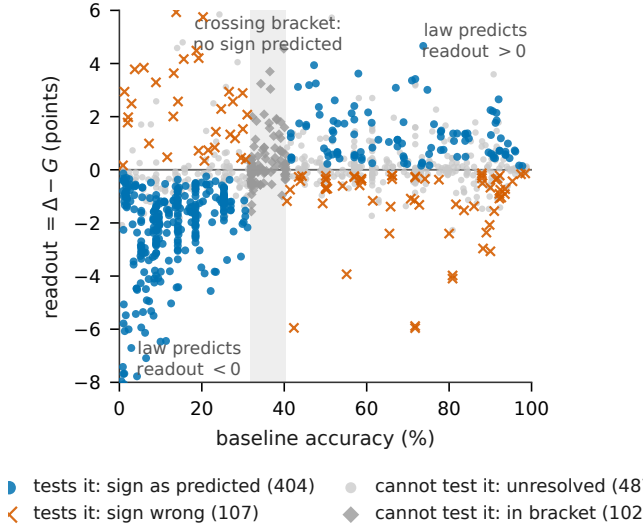
Figure 4: The law, in full: \text{readout} = \Delta - G against baseline accuracy for all 1,100 law-scope cells with \geq 3 seeds on both arms. Shaded band: the measured crossing bracket [31.8, 40.3], inside which no sign is predicted. Of the 511 cells whose readout is resolvable against its own seed-paired uncertainty, 404 fall on the predicted side of zero. The scatter at fixed baseline is substantial ( R^2 = 0.18 , residual SD 2.1 points): the account predicts the sign of this term, not its value.
