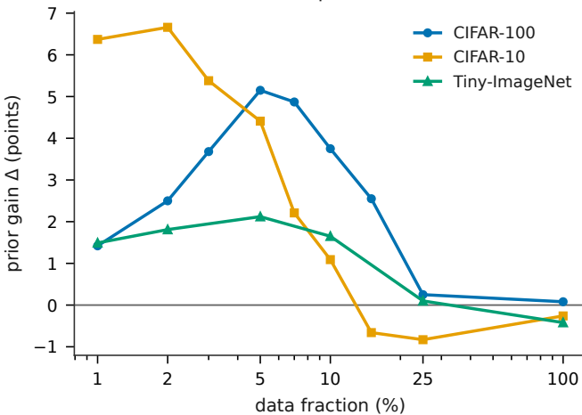
(a) ResNet-18, frozen recipe
