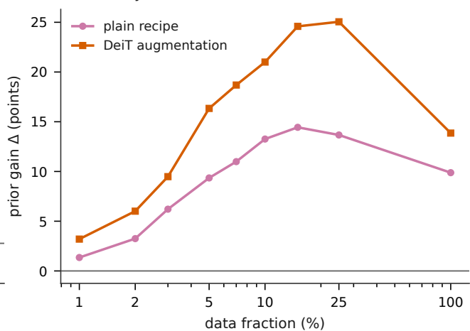
(b) ViT-tiny, CIFAR-100
